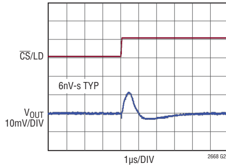
DAC-to-DAC Crosstalk
